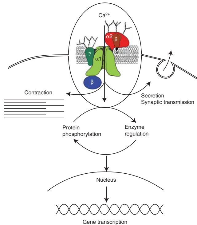
Figure 1. Signal transduction by voltage-gated Ca 2+ channels. Ca 2+ entering cells initiates numerous intracellular events, including contraction, secretion, synaptic transmission, enzyme regulation, protein phosphorylation/dephosphorylation, and gene transcription. ( Inset ) Subunit structure of voltage-gated Ca 2+ channels. The five-subunit complex that forms high-voltage-activated Ca 2+ channels is illustrated with a central pore-forming α1 subunit, a disulfide-linked glycoprotein dimer of α2 and δ subunits, an intracellular β subunit, and a transmembrane glycoprotein γ subunit (in some Ca 2+ channel subtypes). As described in the text, this model is updated from the original description of the subunit structure of skeletal muscle Ca 2+ channels. (Adapted from Takahashi et al. 1987).
