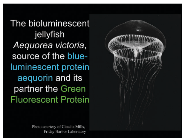
Fig. 2 The jellyfish Aequorea victoria or Aequorea aequorea from which aequorin and Green Fluorescent Protein were isolated. Photo courtesy of Dr Claudia E. Mills, Friday Harbor Laboratories.
